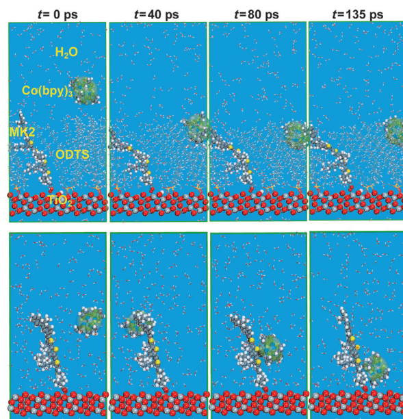
Figure 3. Snapshot of the simulated systems of the ODTS-untreated and treated dyed \text{TiO}_2 cluster as a function of simulation time. In the ODTS-untreated system (bottom), the MK2 molecule was attached on \text{TiO}_2 cluster, whereas the ODTS-treated dyed \text{TiO}_2 photoanode (top) was obtained by attaching the cross-linked hydrolyzed ODTS molecules in the vacant sites. Both systems were immersed in an explicit water environment.
